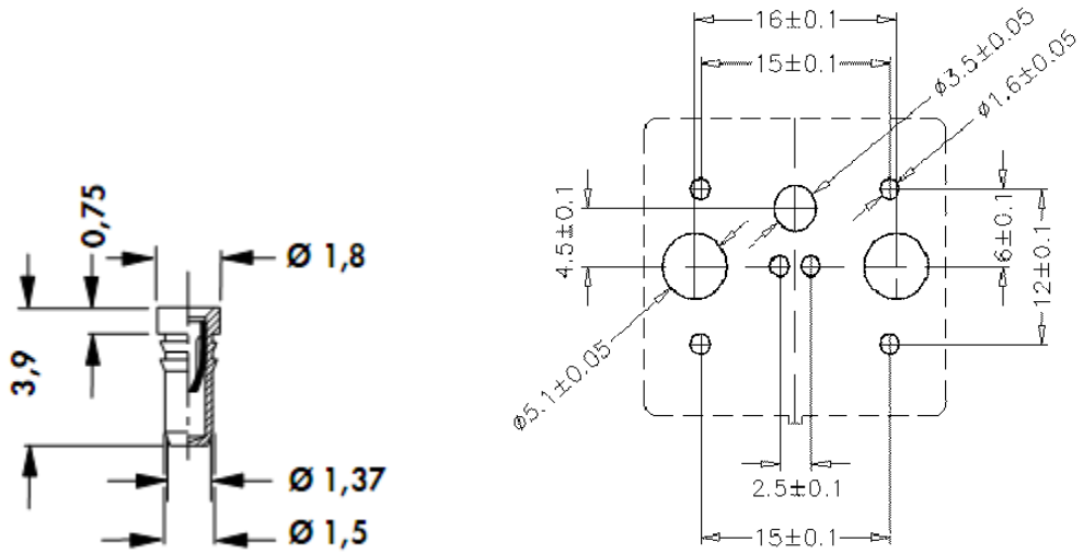
PCB Drill Mask for Socket Pin Mounting of Sxnnn Switches
